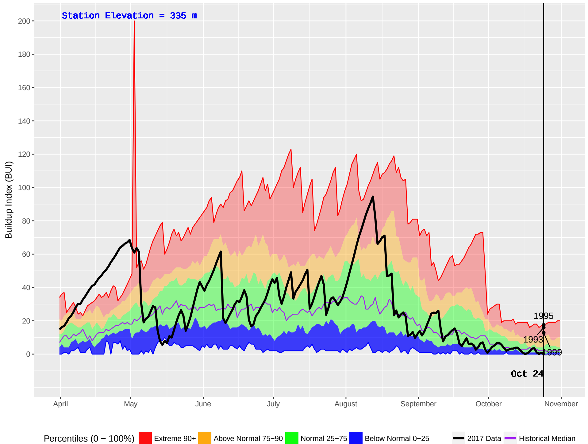
KISPIOX HUB (428) : Historical (1970–2016) and Current (2017) Noon Buildup Index (BUI)
