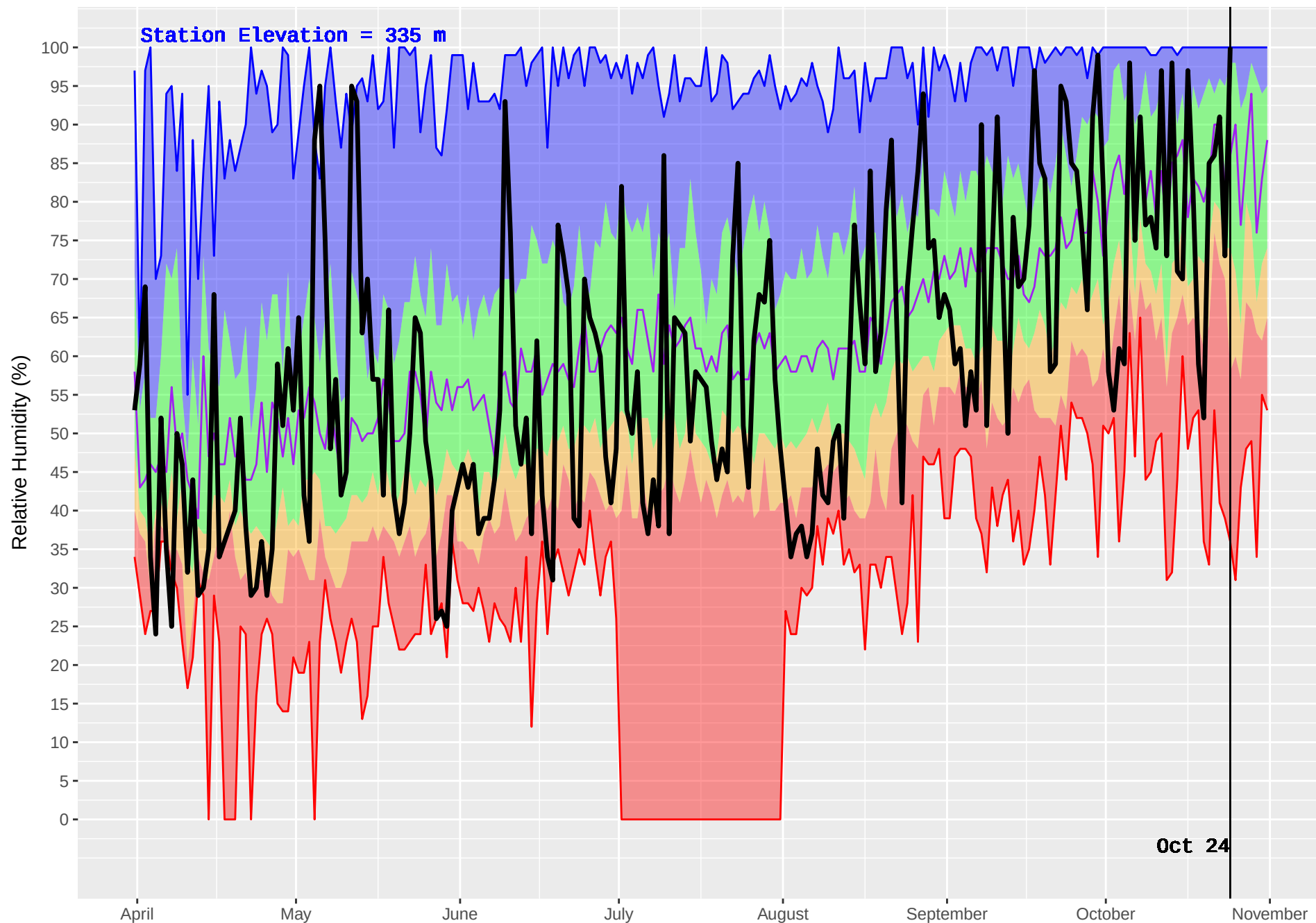
KISPIOX HUB (428) : Historical (1970–2016) and Current (2017) Noon Relative Humidity
